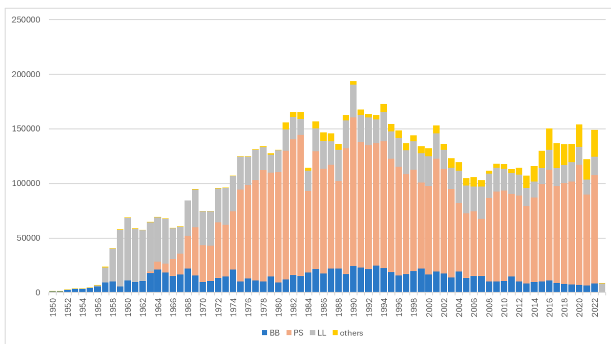
Figure 2. Yellowfin tuna cumulative T1NC catches (t) by major gear between 1950 and 2023* (*2023 is provisional and incomplete).
