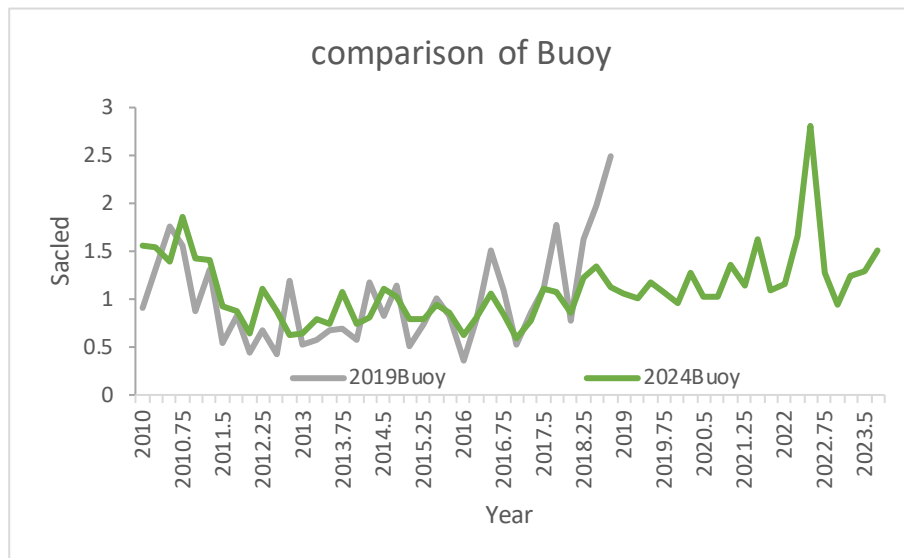
Figure 11. Comparison of the yellowfin tuna Bouy derived index of abundance from the FOBs deployed by the EU PS fleets.
