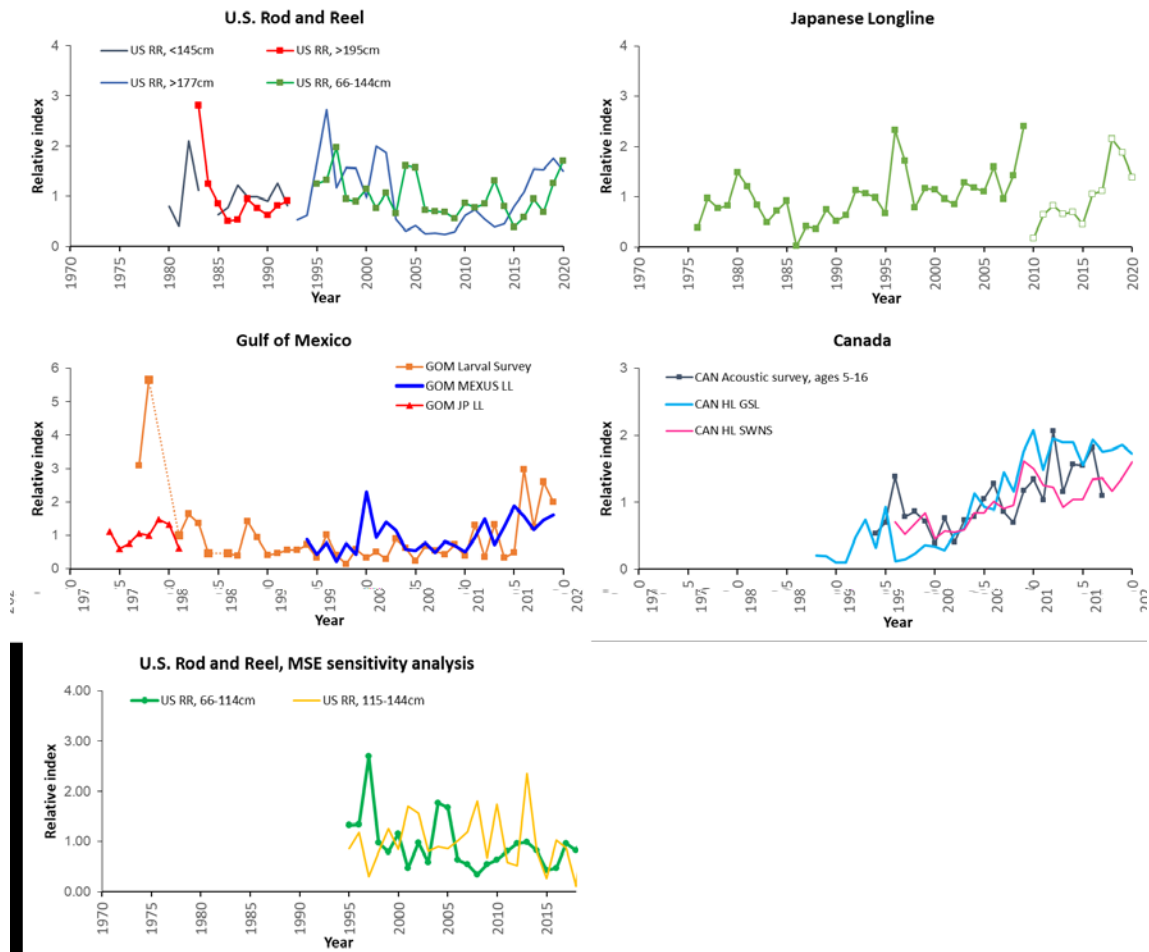
Figure 3. Abundance indices for W-BFT for the 2021 W-BFT stock assessment and the MSE.
