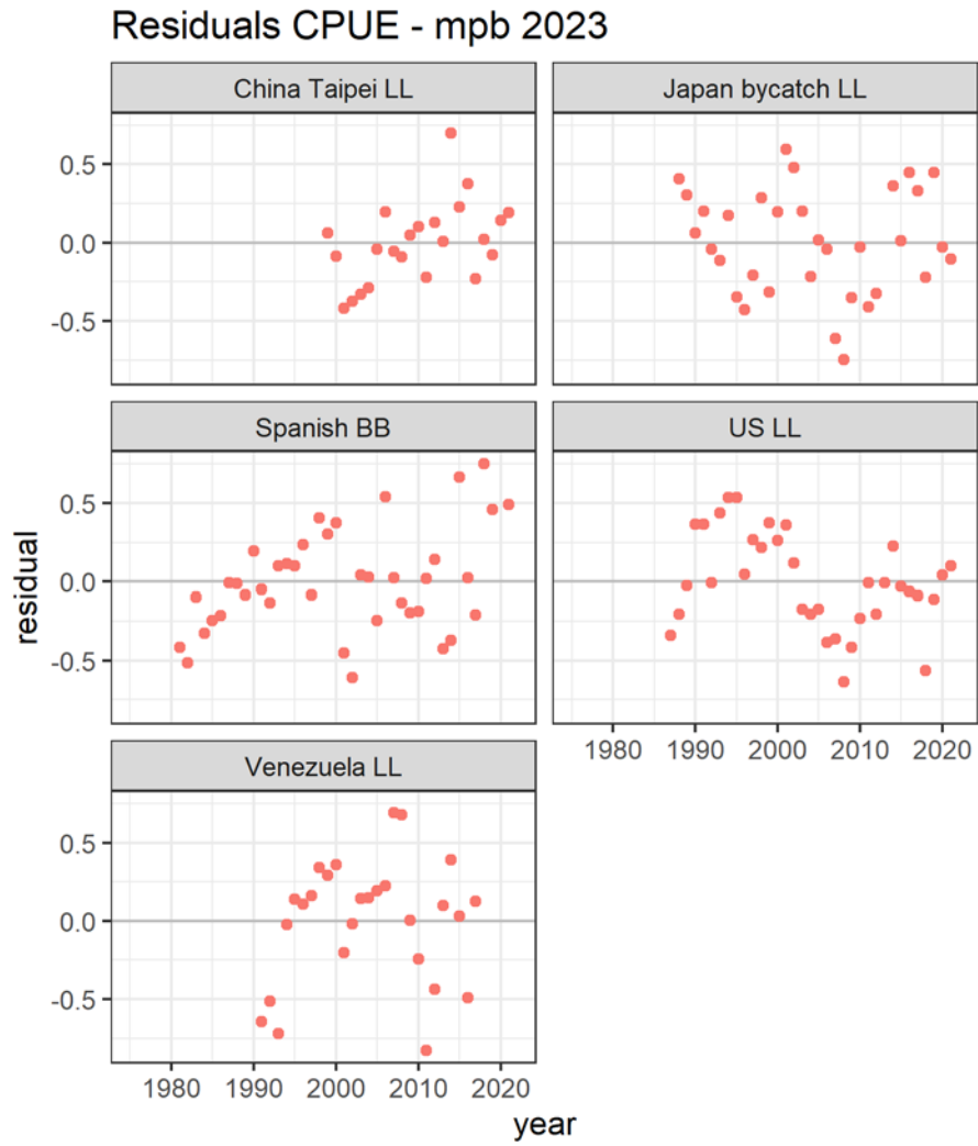
Figure 18. Time series of residuals of fit for each of the five indices available for this stock assessment.
