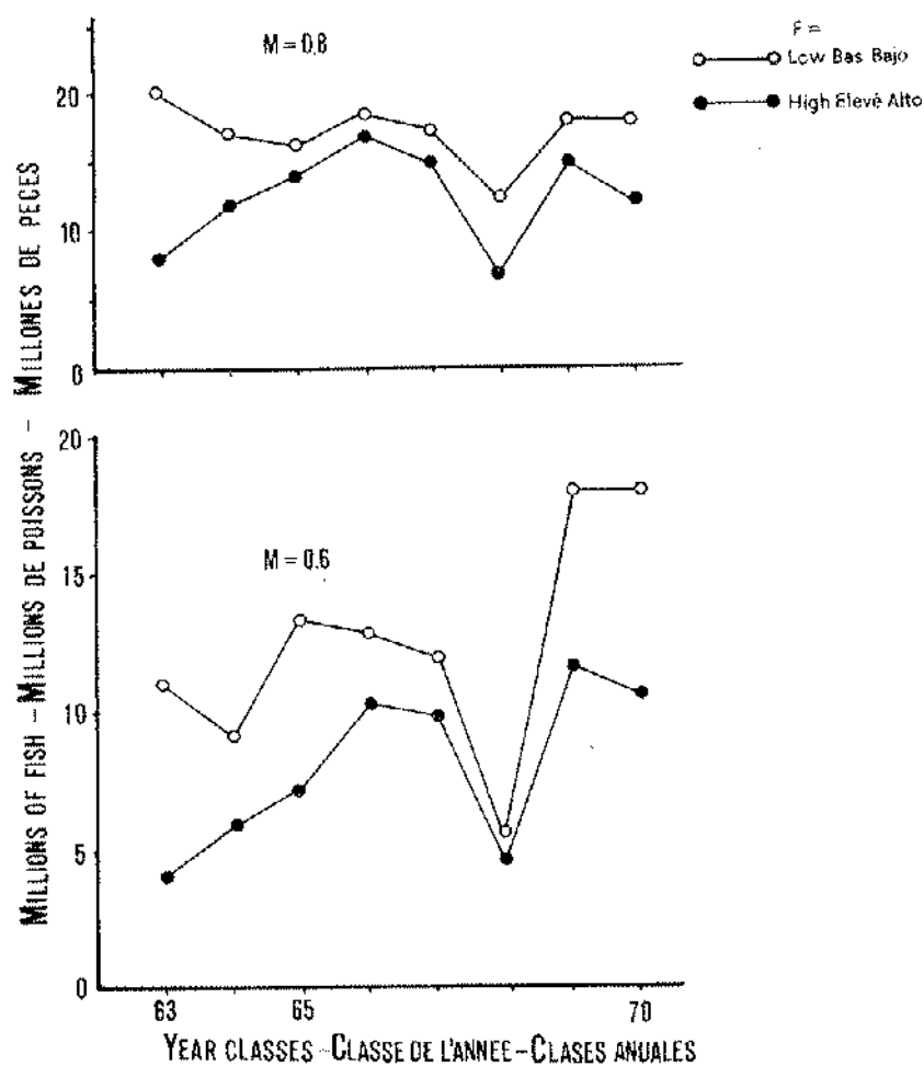
FIG. 2. Yearly fluctuation of yellowfin year classes.
