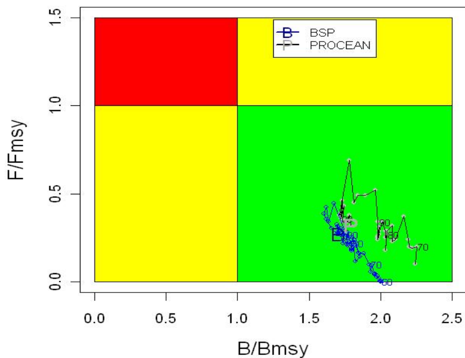
SKJ-Figure 14. Eastern skipjack stock status: trajectories of B/B_{MSY} and F/F_{MSY} from the Bayesian surplus production model (Schaefer type), and from the generalized multi-fleets dynamic model.
