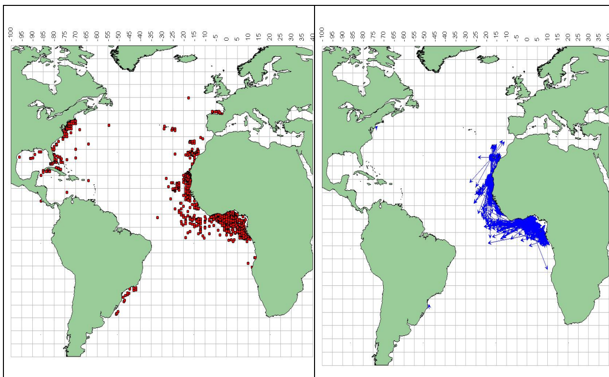
SKJ-Figure 10. Distribution of tagged and released SKJ (left panel) and apparent movement from geographic positions of recaptured fish (right panel).
