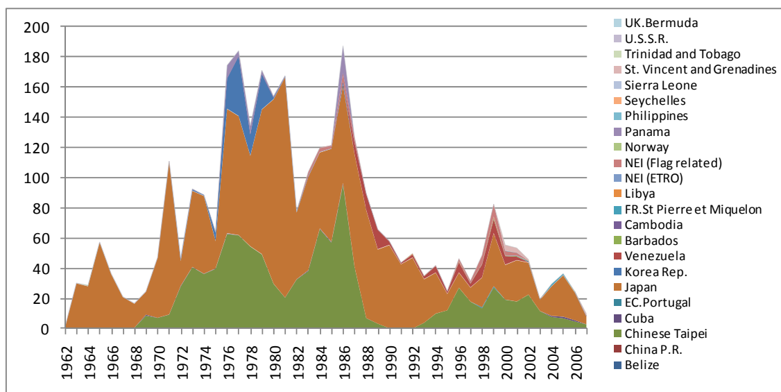
SHK-Figure 2. Estimated potential catch of porbeagle by non-reporting longline fleets using catch ratios for the northwest stock. Limited observations across the time-series result in an unquantified uncertainty in the estimates.
