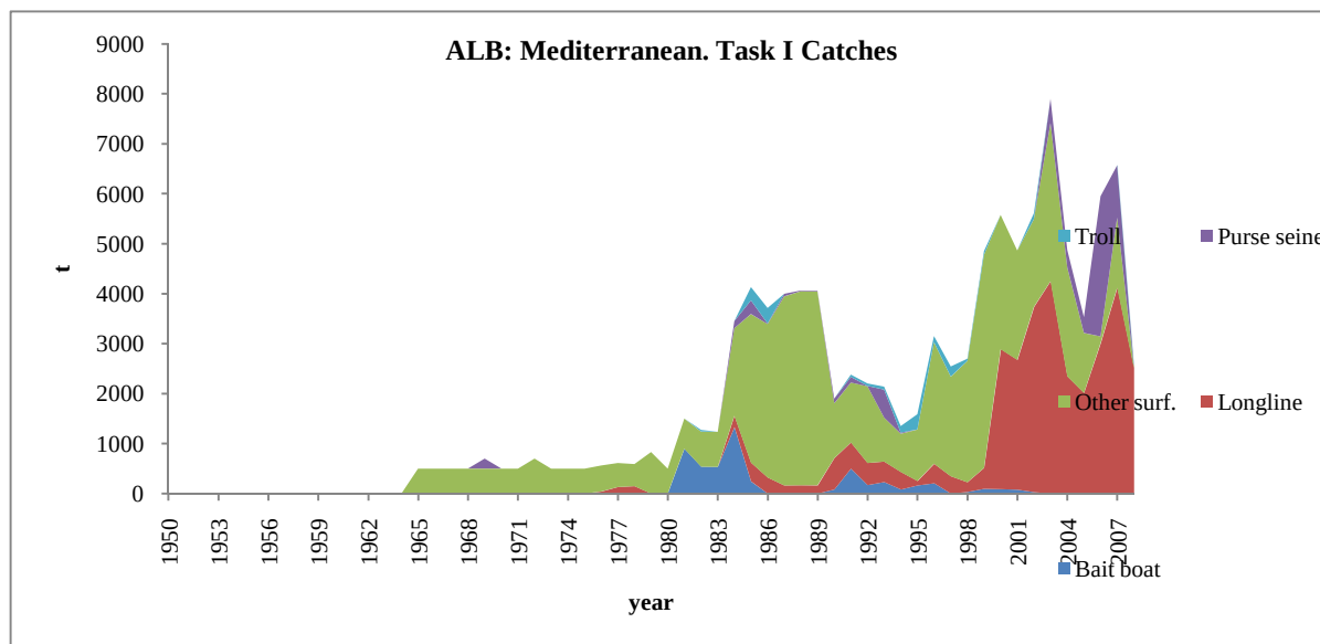
ALB-Figure 2a, b, c. Total albacore catches reported to ICCAT (Task I) by gear for the northern, southern Atlantic stocks including TAC, and the Mediterranean stock.
