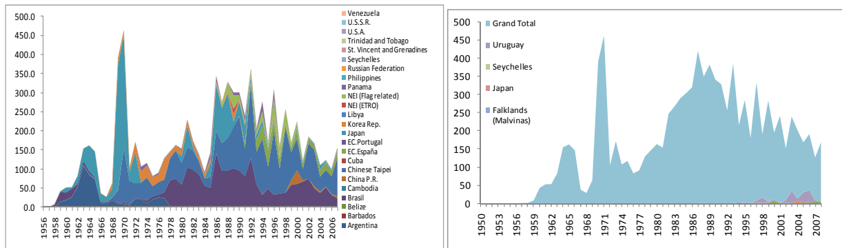
SHK Figure 3. Left plate: Estimated potential catch of porbeagle by non-reporting longline fleets using catch ratios for the southwest stock. Very limited observations across the time-series result in a high but unquantified uncertainty in the estimates. Right plate: Comparison of estimates for non-reporting longline fleets with reported catch levels held in the Task I data set for the southwest stock area.
