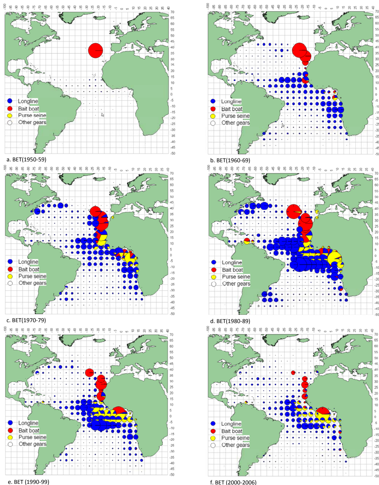
BET-Figure 1. Historical development of the area distribution of bigeye catches by fishing gear. The most recent period (2000-2006) is shown in the bottom right panel. Ghana's catches have been included in the same 5x5° square, as no detailed information on the spatial distribution of these catches is available.
