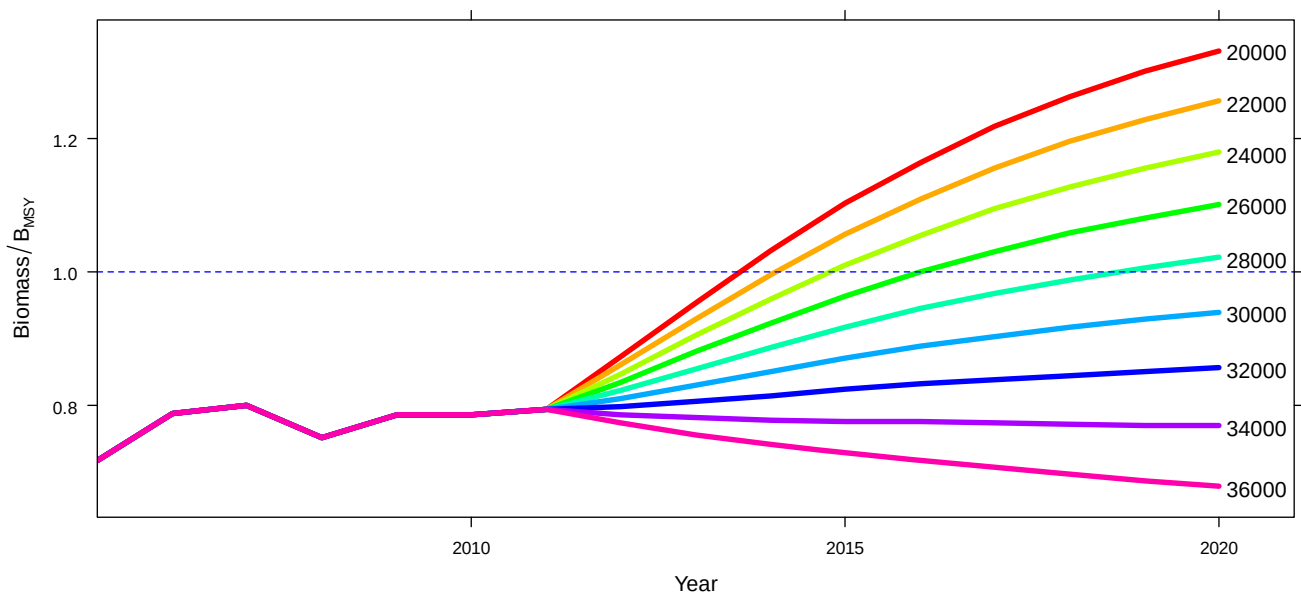
ALB-Figure 11. Estimated projections of relative SSB ( SSB/SSB_{MSY} ) for different scenarios of constant catch (20,000 t-36,000 t) assuming average recent year-class strengths for the North Atlantic albacore stock.
