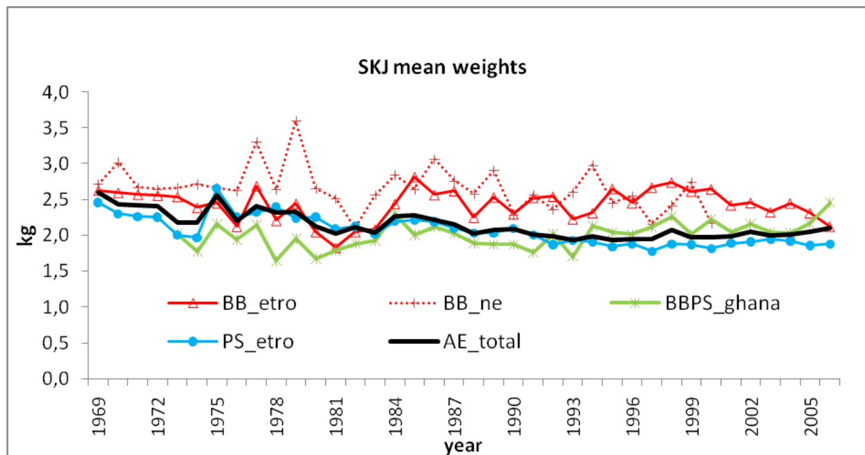
SKJ-Figure 8. Changes in time of the mean weight of the skipjack landed (non standardized) by major fisheries in the eastern Atlantic.
