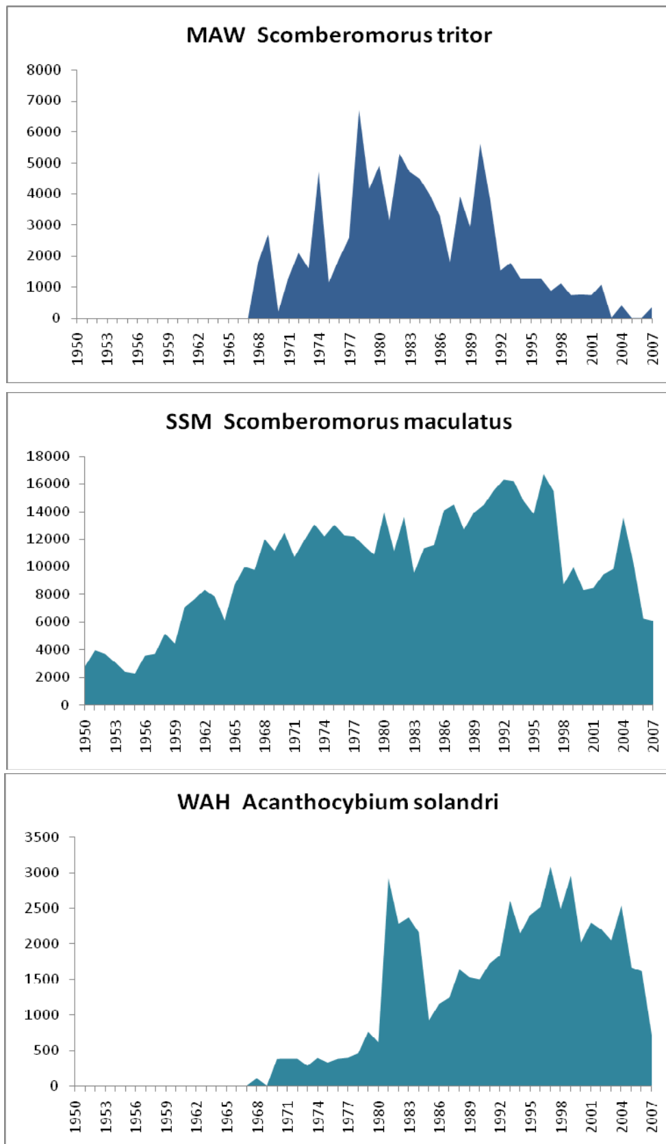
SMT-Figure 2. Estimated landings (t) of the major species of small tunas in the Atlantic and Mediterranean, 1950-2007. The data for the last years are incomplete.
