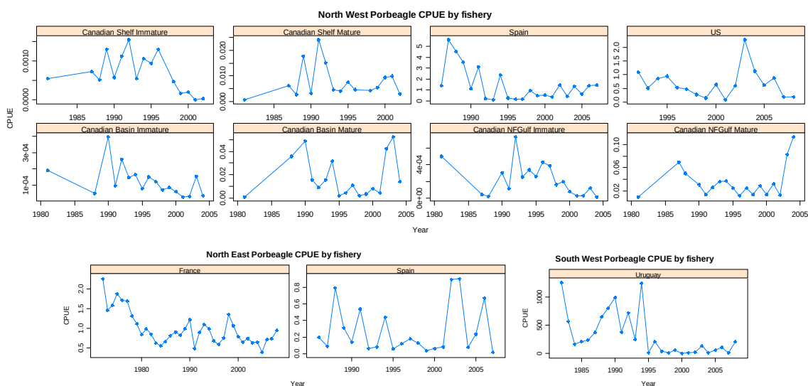
SHK-Figure 6. CPUE series for the porbeagle northwest stock (upper figures), northeast stock (lower left figures) and southwest stock (lower right figure).
