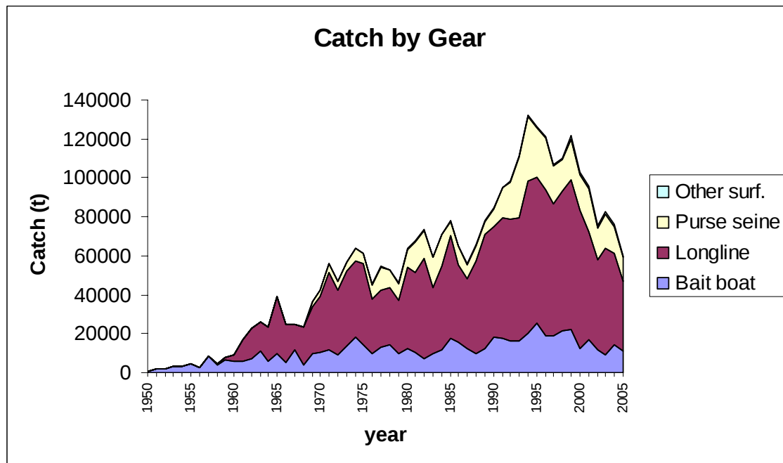
BET-Figure 1. Trend of bigeye catches (1950-2005) by major tuna fishery.
