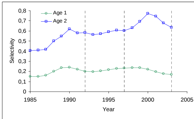
Figure 15.7.3 Estimated trend in selectivity ( F at age scaled to the maximum F at age for each year) for age 1 and age 2 northern Atlantic swordfish since 1985 until the year for which we have reliable estimates for these year classes. Also indicated as vertical lines are years in which Commission recommendations affecting minimum size or TAC became fully effective.
