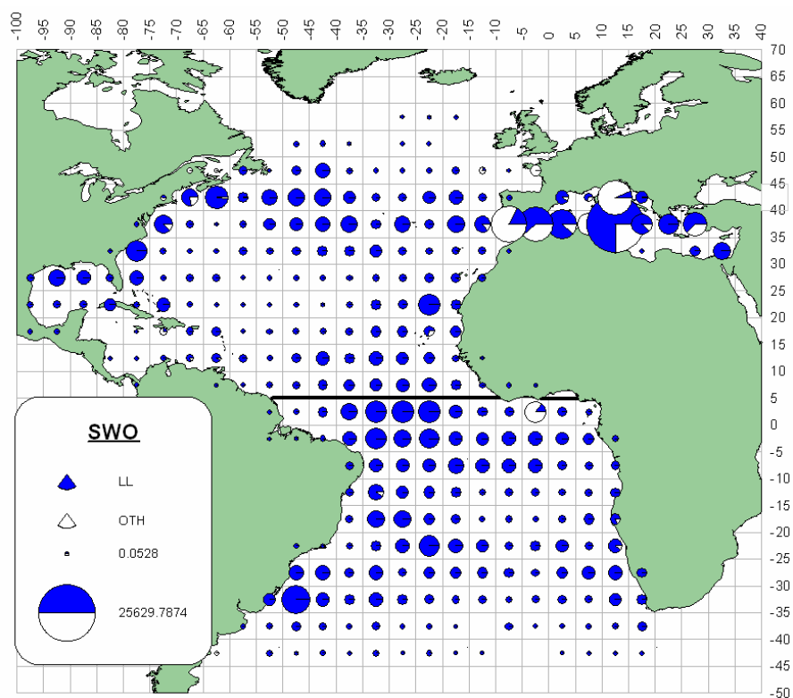
SWO Figure 1. Geographical distribution of swordfish cumulative catch (t) by gear, for the period 2000-2004 in the Convention area.
