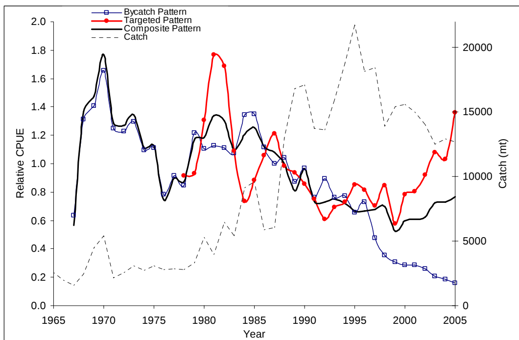
SWO-ATL Figure 5. Relative CPUE patterns from bycatch (Japan and Chinese Taipei) and targeted (Brazil and EC-Spain) fleets harvesting southern Atlantic stock swordfish compared to catch of southern Atlantic swordfish.
