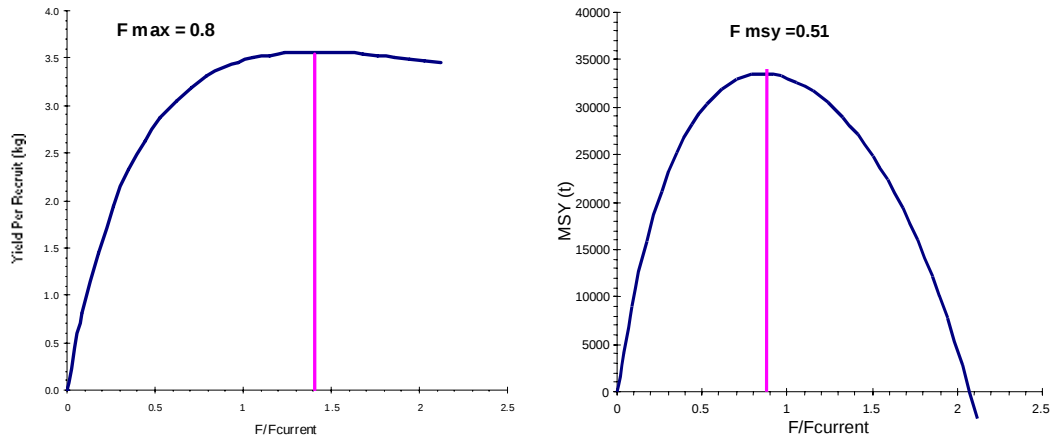
ALB-Figure 5. Yield-per-recruit (left) and equilibrium yield (right) estimated by the 2000 VPA for the northern albacore stock. Fishing mortality (x-axis) is relative to current fishing mortality ( F_{1999} = 0.57 ).
